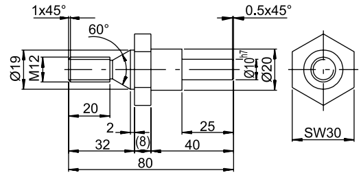
Wellenadapter M12
