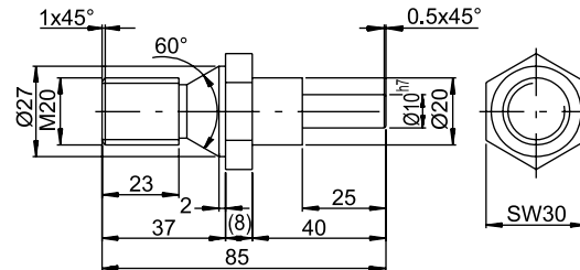
Wellenadapter M20
