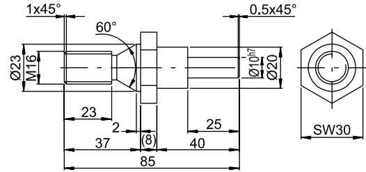
Wellenadapter M16
